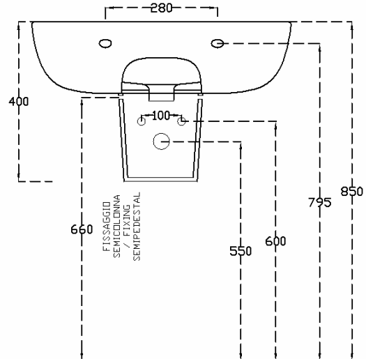
LAVABO (M15) + SEMICOLONNA (M22) WASHBASIN (M15) + SEMIPEDESTAL (M22)
